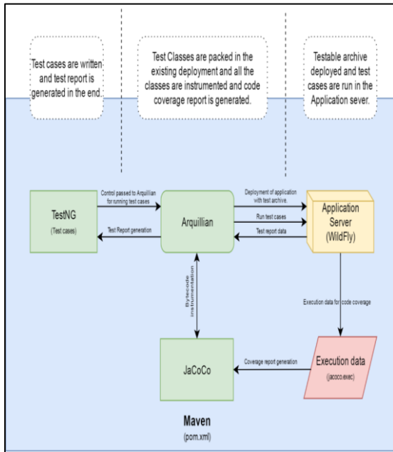
Fig 2: Architecture of in Container Integration Frame
